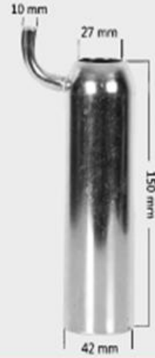
DD16/1 PASLANMAZ KILIF 1./STAINLESS STEEL LINER CUP 1.
